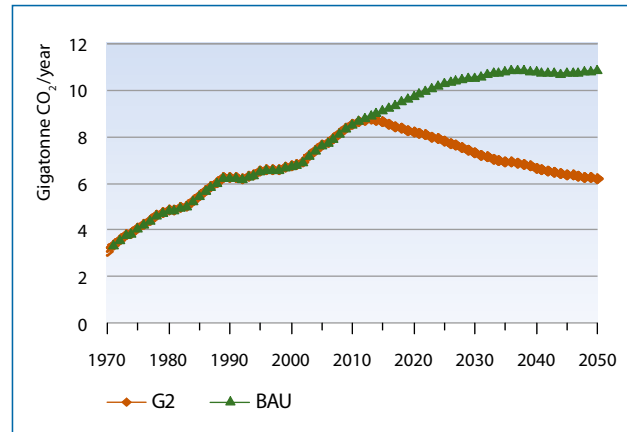
Figure 6: Total CO 2 emissions per year in buildings sector 2010–2050
