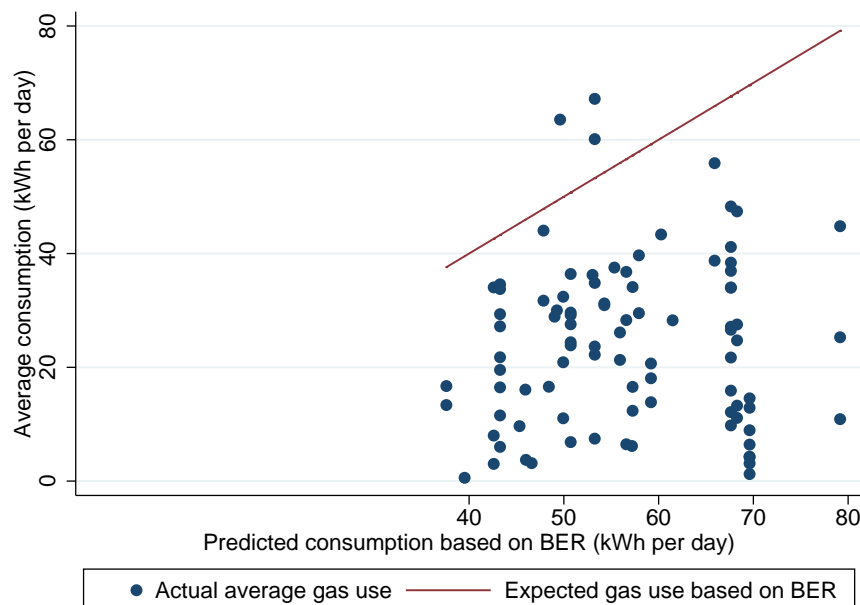
Fig. 2 Comparison of predicted heating demand based on each dwelling's BER (BERpred) with average actual gas use per day; results are included both before and after upgrades for households that received them. BERpred includes the electricity used for lighting and ventilation in addition to the gas used for heating
