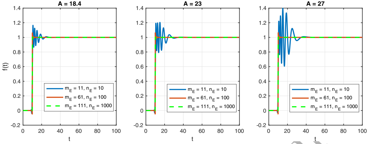
Figure 2: Output of the inverse Laplace transform of \tilde{f}(s) = \frac{e^{-10s}}{s} . Increasing m_E and n_E reduces the size of the oscillations, but it is not improved by increasing A .
