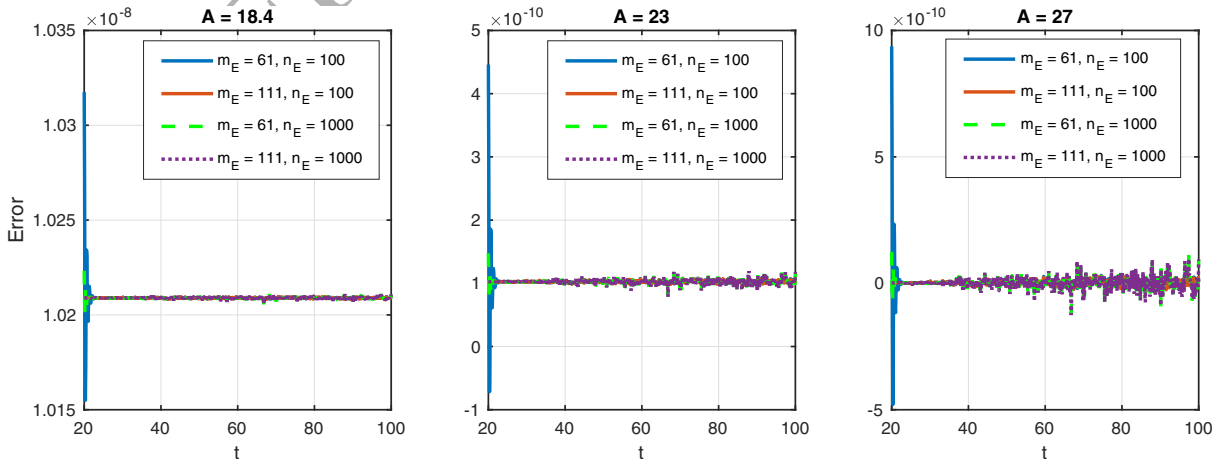
Figure 4: Error of the inverse Laplace transform of \tilde{f}(s) = \frac{e^{-10s}}{s} . Increasing A decreases the error floor, while the latter is unaffected by increasing m_E and n_E . The noise on the error floor is \approx 10^{-10} .
