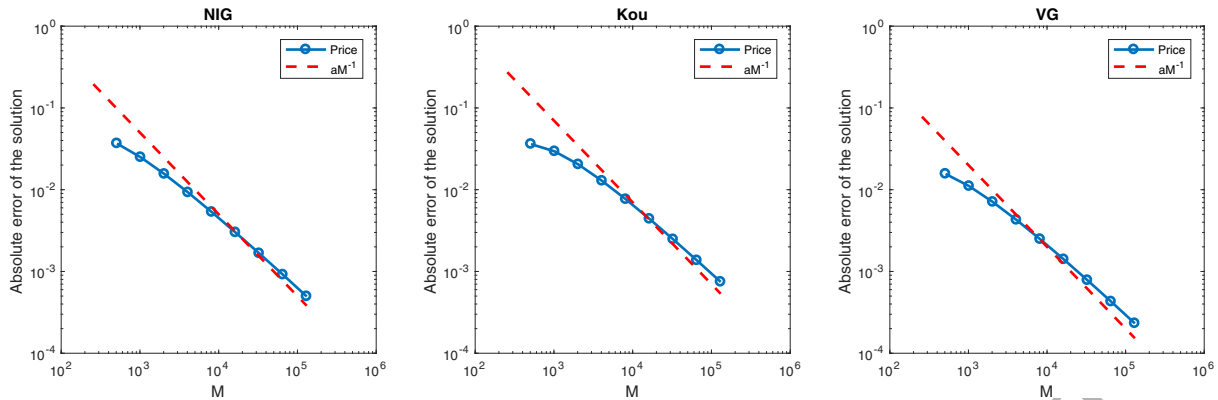
Figure 8: Error convergence for the continuously monitored double-barrier option. The absolute error is worse than that for the single-barrier option, but the error convergence conforms to the calculated error bound.
