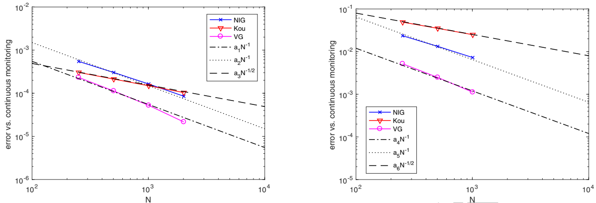
Figure 9: Error for discretely monitored barrier options used as an approximation of the price for the continuously monitored case, plotted as a function of the number of monitoring dates. The error is calculated as the difference between the prices for discrete and continuous monitoring at the maximum grid size of 2^{17} . Results for single and double-barrier options are displayed on the left and right hand plots respectively. Notice that the error for the Kou process converges as O(1/\sqrt{N}) , whereas the error for the NIG and VG processes converges a rate of approximately O(1/N) .
