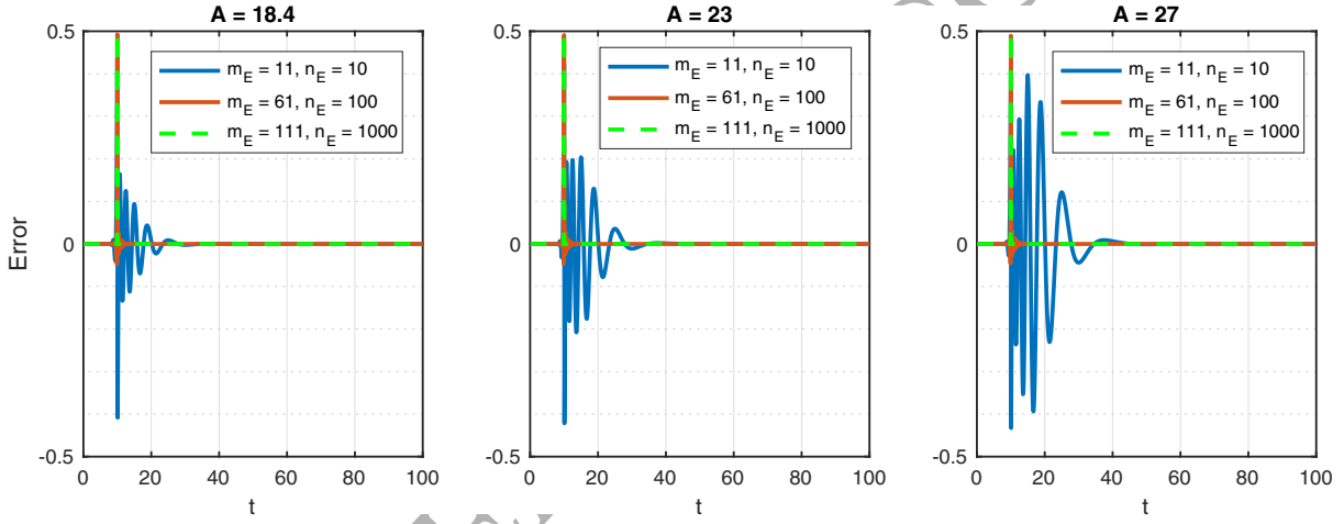
Figure 3: Error of the inverse Laplace transform of \tilde{f}(s) = \frac{e^{-10s}}{s} . Increasing m_E and n_E reduces the size of the errors due to the oscillations, but it is not improved by increasing A .
