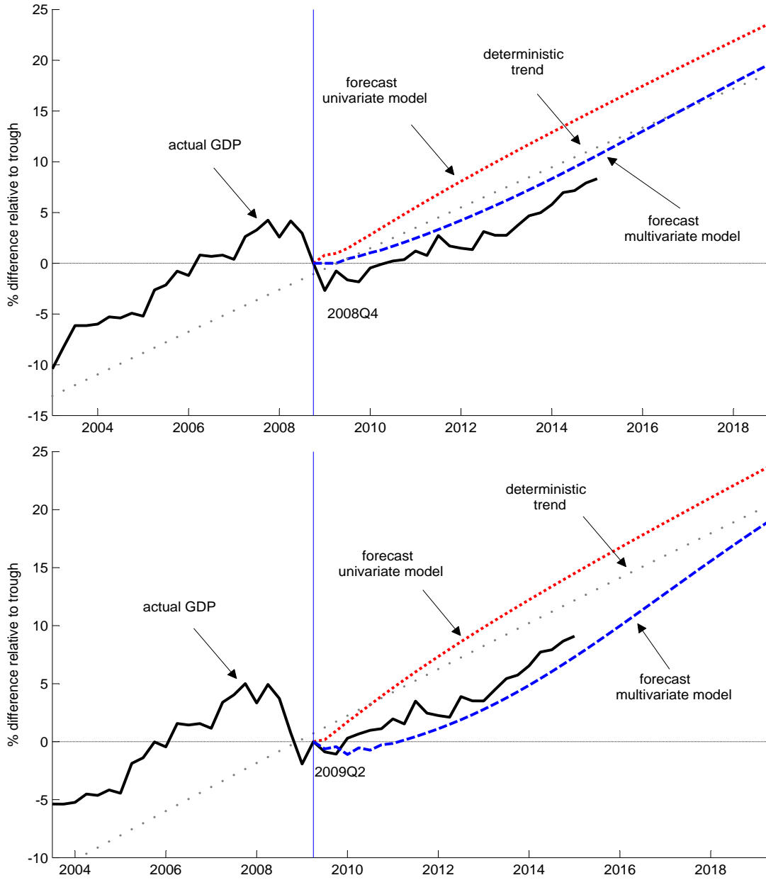
Figure 8: The start and trough of the great UK recession
