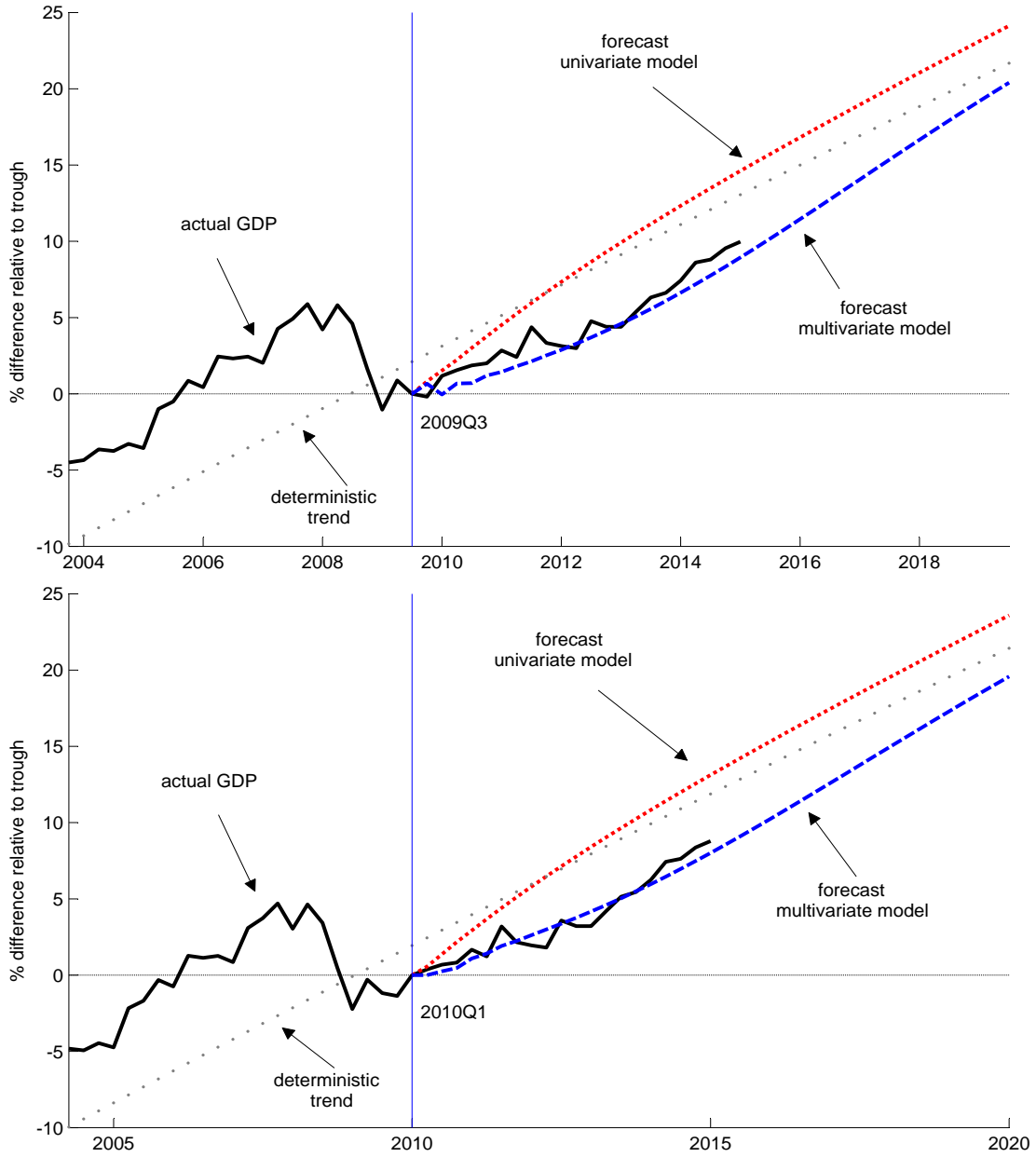
Figure 9: The initial recovery of the great UK recession
