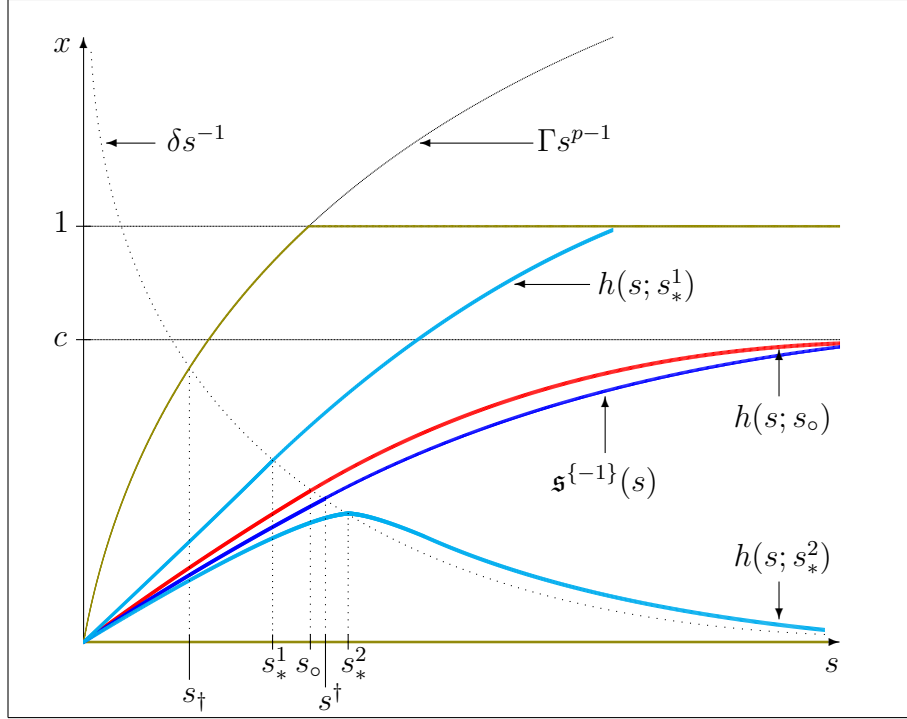
Figure 5 ( p > 1 ) Illustration of the proof of Lemma 2.(II) for s_o(\delta) = s^\circ(\delta) . The identity h(s; s_*) = s^{-1}H(s; s_*) for all s > 0 relates the solutions to (61) for s_* = s_*^1, s_o, s_*^2 plotted here with the solutions to the ODE (23) satisfying (26) that are plotted in Figure 3. Furthermore, the intersection of \mathbb{R}^2 with the boundary of the domain \mathcal{D}_h^2 in which we consider solutions to (61) is designated by green.
