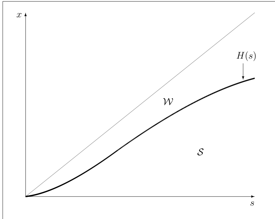
Figure 1 Depiction of the free-boundary function H separating the stopping region \mathcal{S} from the waiting region \mathcal{W} .
