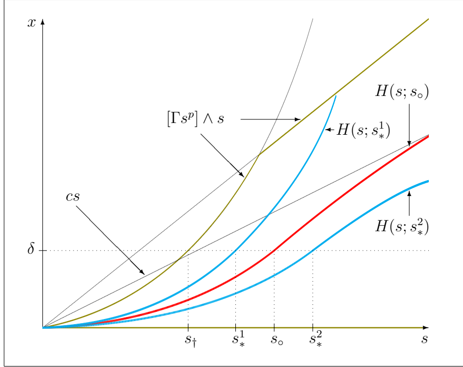
Figure 3 ( p > 1 ) Illustration of Lemma 2.(II) for s_0(\delta) = s^\circ(\delta) . The free-boundary function H(\cdot) = H(\cdot; s_0) that separates the stopping region \mathcal{S} from the waiting region \mathcal{W} is plotted in red. The intersection of \mathbb{R}^2 with the boundary of the domain \mathcal{D}_H in which we consider solutions to the ODE (23) satisfying (26) is designated by green. Every solution to the ODE (23) satisfying (26) with s_* \in ]s_\dagger, s_0[ (resp., s_* > s_0 ) hits the upper part of the boundary of \mathcal{D}_H in the picture (resp., has asymptotic growth as s \rightarrow \infty that is of different order than the one of the free-boundary): such solutions are plotted in blue.
