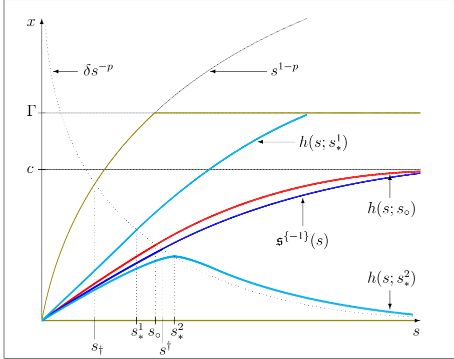
Figure 4 ( p < 1 ) Illustration of the proof of Lemma 2.(I) for s_o(\delta) = s^\circ(\delta) . The identity h(s; s_*) = s^{-p}H(s; s_*) for all s > 0 relates the solutions to (55) for s_* = s_*^1, s_o, s_*^2 plotted here with the solutions to the ODE (23) satisfying (26) that are plotted in Figure 2. Furthermore, the intersection of \mathbb{R}^2 with the boundary of the domain \mathcal{D}_h^1 in which we consider solutions to (55) is designated by green.
