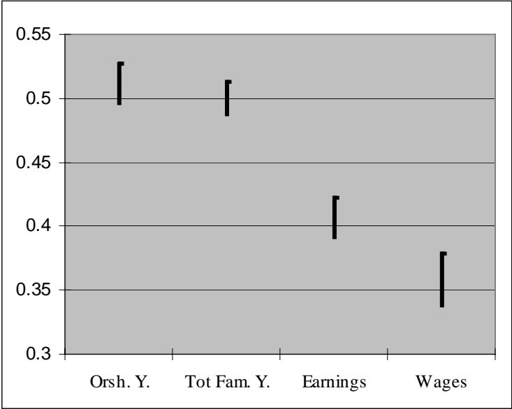
Figure 1: Range of estimates of \beta derived from the averaging estimator
