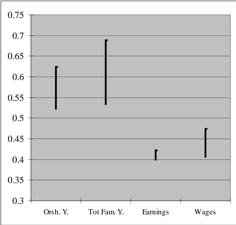
Figure 2: Range of estimates of \beta derived from the modified OLS estimator
