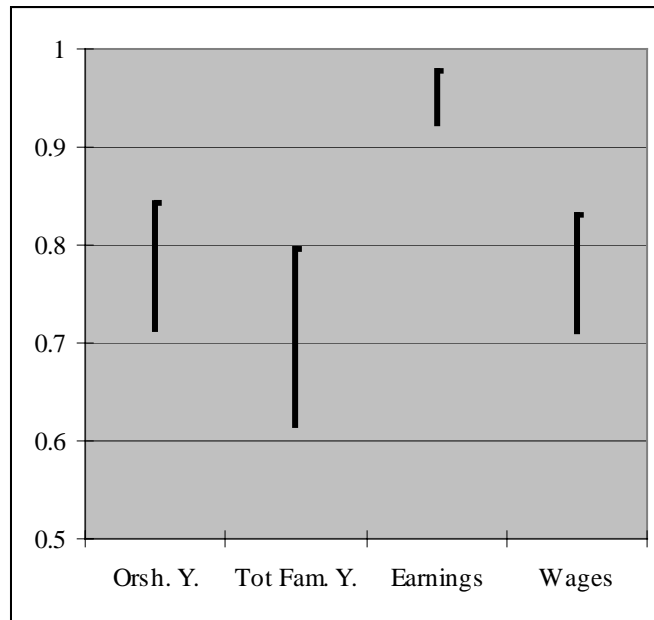
Figure 3: Range of estimates of \lambda , the signal to total variance ratio
