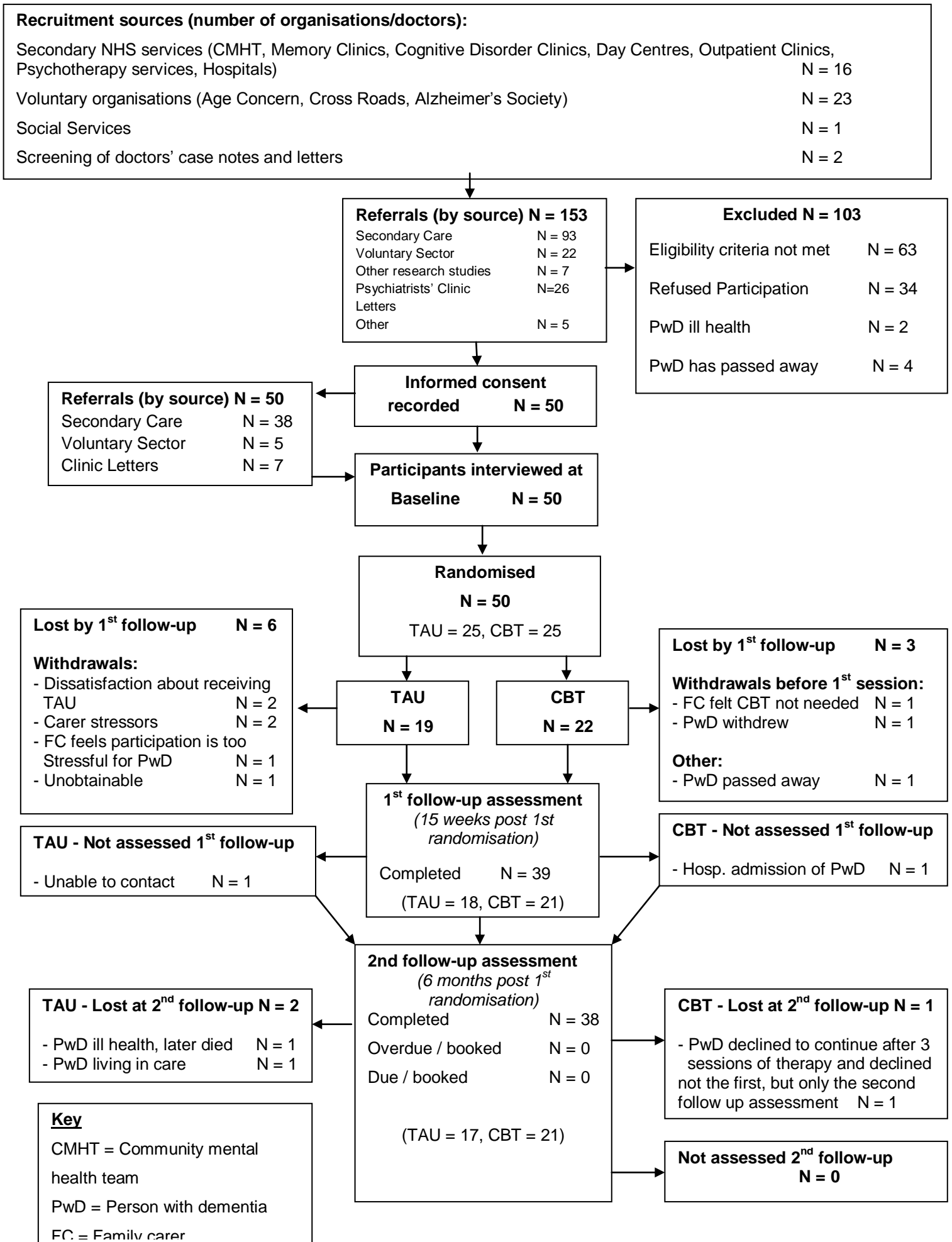
Figure 1: CONSORT Diagram
