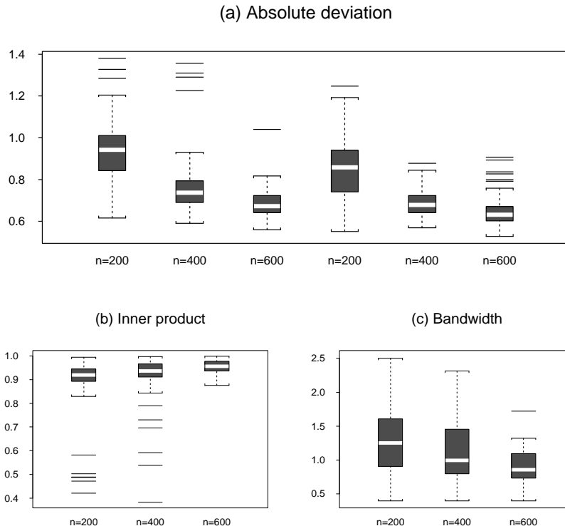
Figure 3: Simulation results for Example 2. Boxplots of (a) \mathcal{E}_{\text{MAD}} , (b) |\beta^T \hat{\beta}| , and (c) the selected bandwidths. The three panels on the left in (a) are based on \hat{\beta} , and the three panels on the right are based on the true \beta .
