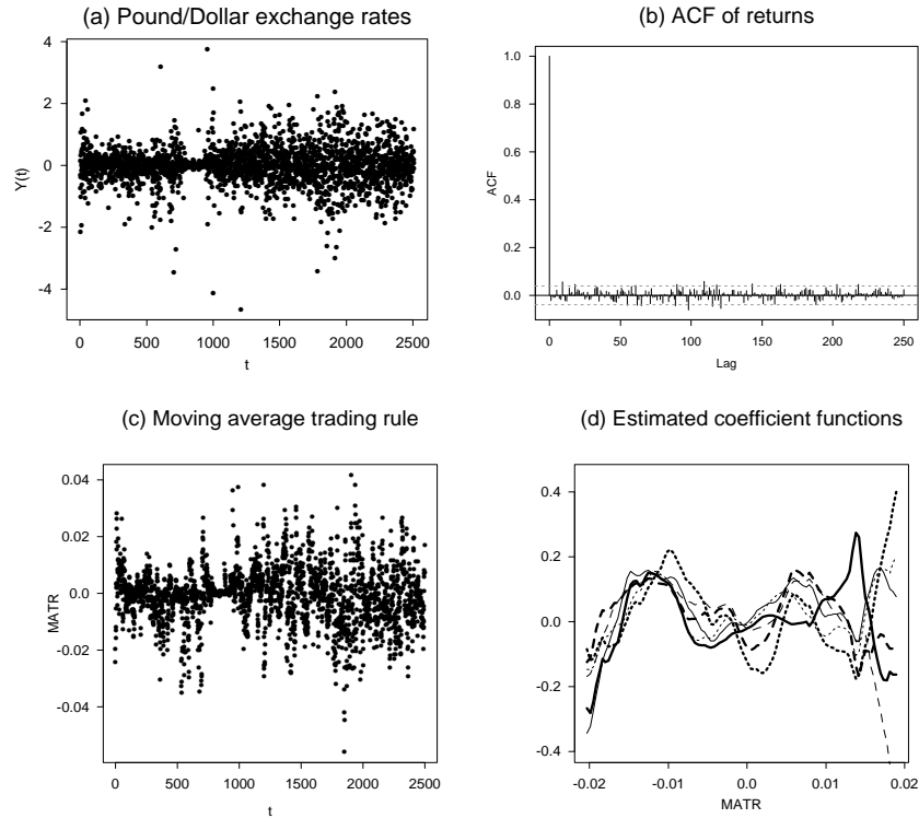
Figure 6: (a) Pound/Dollar exchange rate return series \{Y_t\} . (b) Autoregressive function of \{Y_t\} . (c) Plot of \{U_t = Y_t / (\sum_{i=0}^9 Y_{t-i} / 10)\} . (d) Estimated coefficient functions of model (4.6) with Z_t = U_{t-1} and m = 5 . Thick solid lines — g_0(\cdot) , thick dotted lines — g_1(\cdot) , thick dashed lines — g_2(\cdot) , solid lines — g_3(\cdot) , dotted lines — g_4(\cdot) , dashed lines — g_5(\cdot) .
