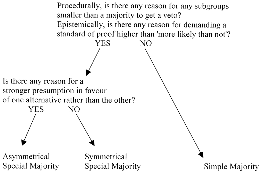
Fig. 2. Grounds for choosing among decision rules
