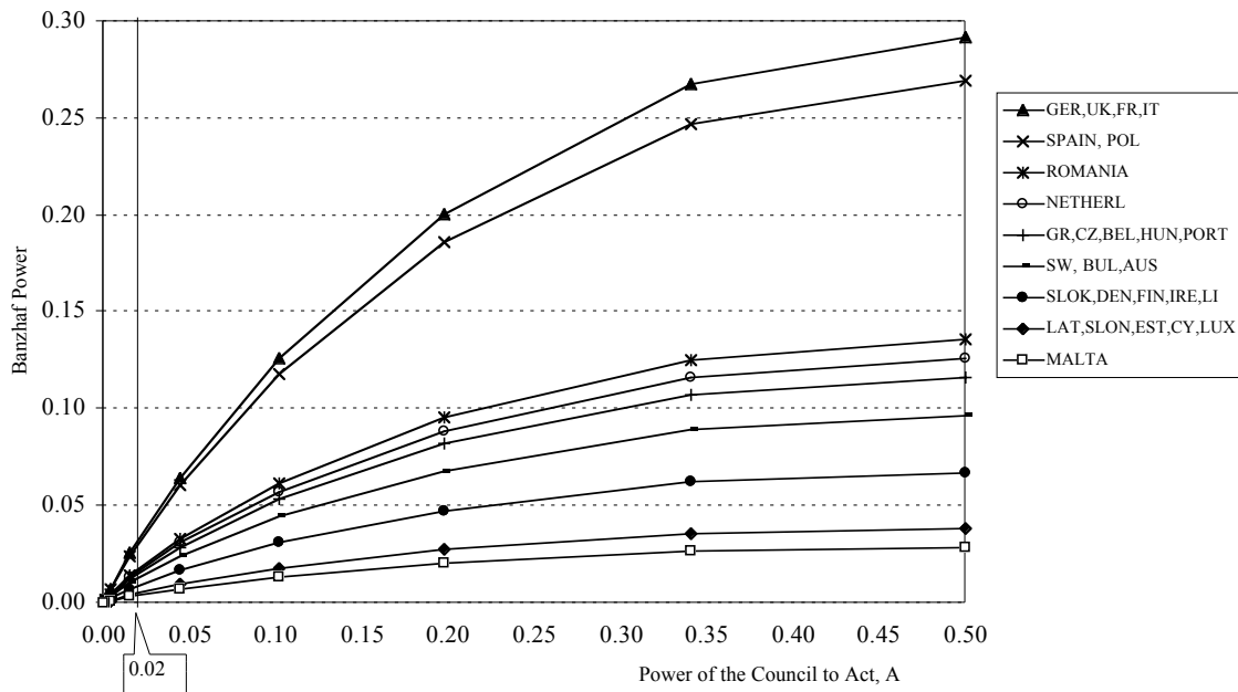
Figure 7: Voting Power \pi_i v. Power to Act A in the European Council EU27
