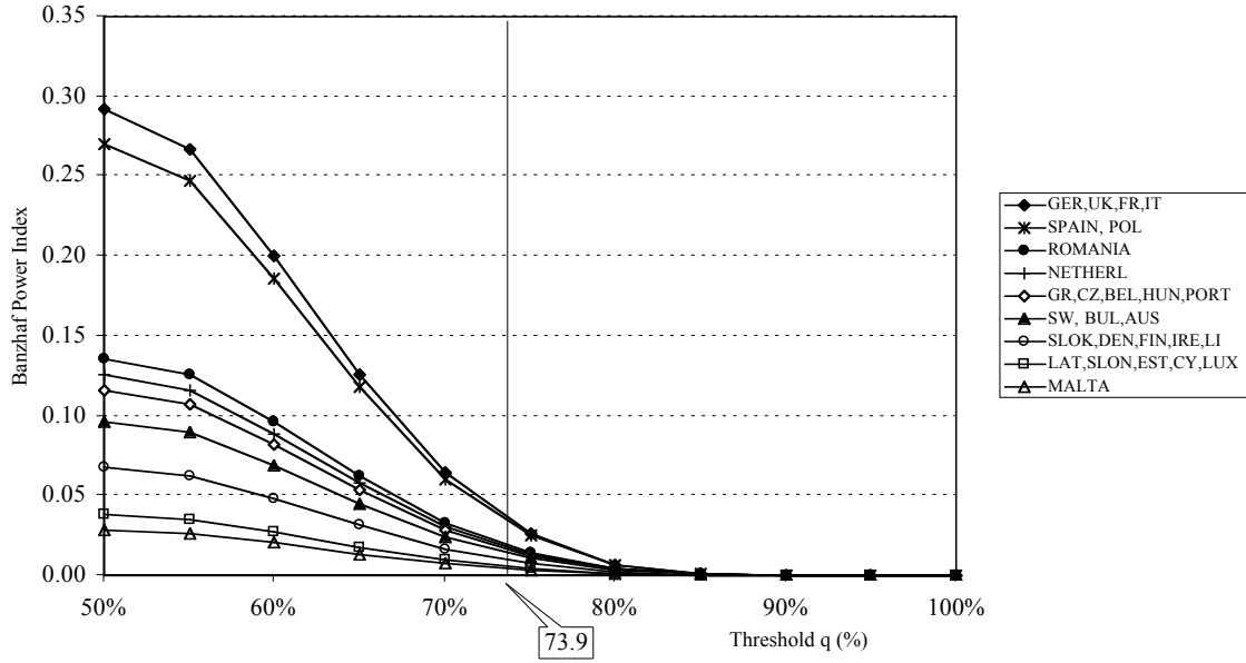
Figure 6: Voting Power \pi_i v. the Threshold q in the European Council EU27
