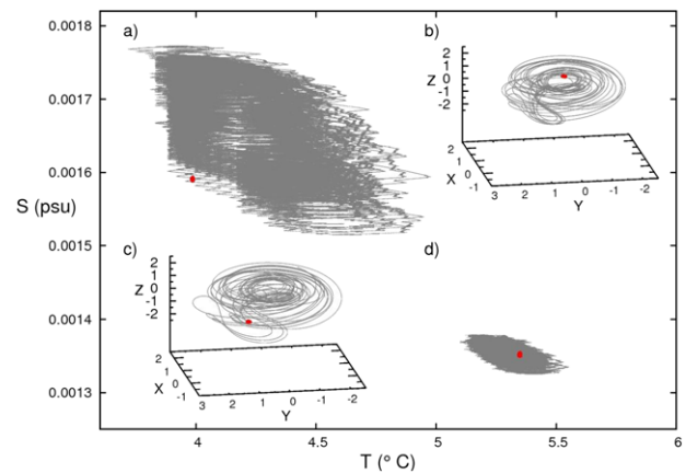
Figure 1. Trajectories of the L84-S61 model: ocean variables (latitudinal temperature ( T ) and salinity ( S ) differences) on the main axes, atmospheric variables ( X , Y , Z ) on insets. Ocean variables show 10 000 year simulations; atmospheric variables a single year. (a) and (b) show trajectories for F_m = 7 while (c) and (d) show trajectories for F_m = 8 . Red points show the IC locations of 10 000 member ensembles. For single ocean variable time series see supplementary figure S3 (available at stacks.iop.org/ERL/8/034021/mmedia ) ( F_m = 7 ) and figure S4 (available at stacks.iop.org/ERL/8/034021/mmedia ) ( F_m = 8 ).
