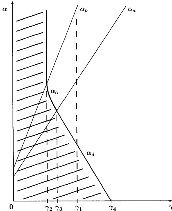
Figure 2: The equilibrium (0, 0)
