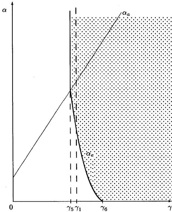
Figure 3 : The equilibrium (1, 1)
