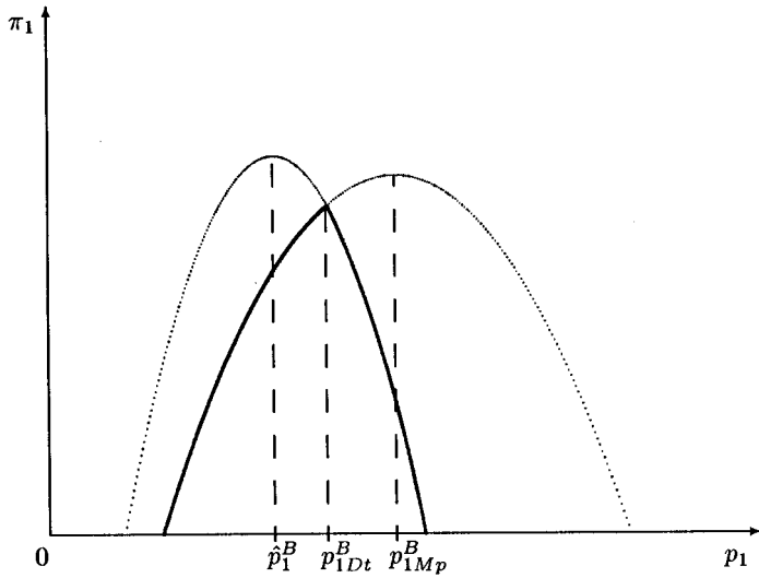
Figure 1a : Firm 1's profit function for \alpha_a < \alpha \leq \alpha_b (bold line).
