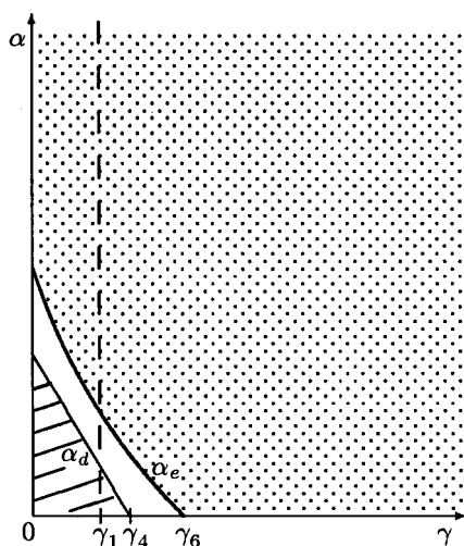
Figure 6 : Analysis of equilibria : Case 3
