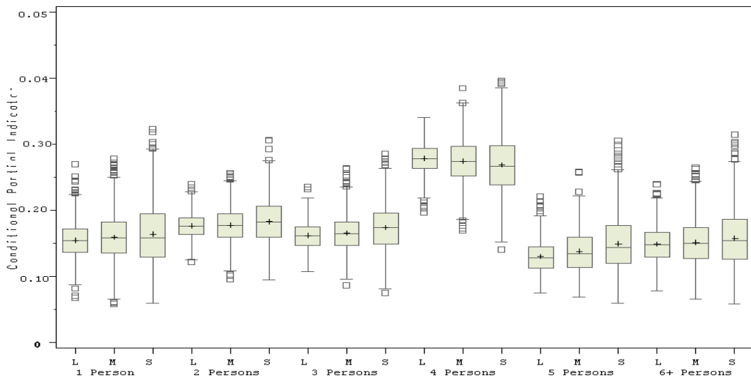
Figure 3.8: Conditional partial indicator P_c(Z = k, \rho_x) for categories of number of persons in the household for three sampling fractions (1:50 (L), 1:100 (M) and 1:200(S)) Population values are: 1 = 0.0155, 2 = 0.0174, 3 = 0.0158, 4 = 0.0289, 5 = 0.0121, 6+ = 0.0147
