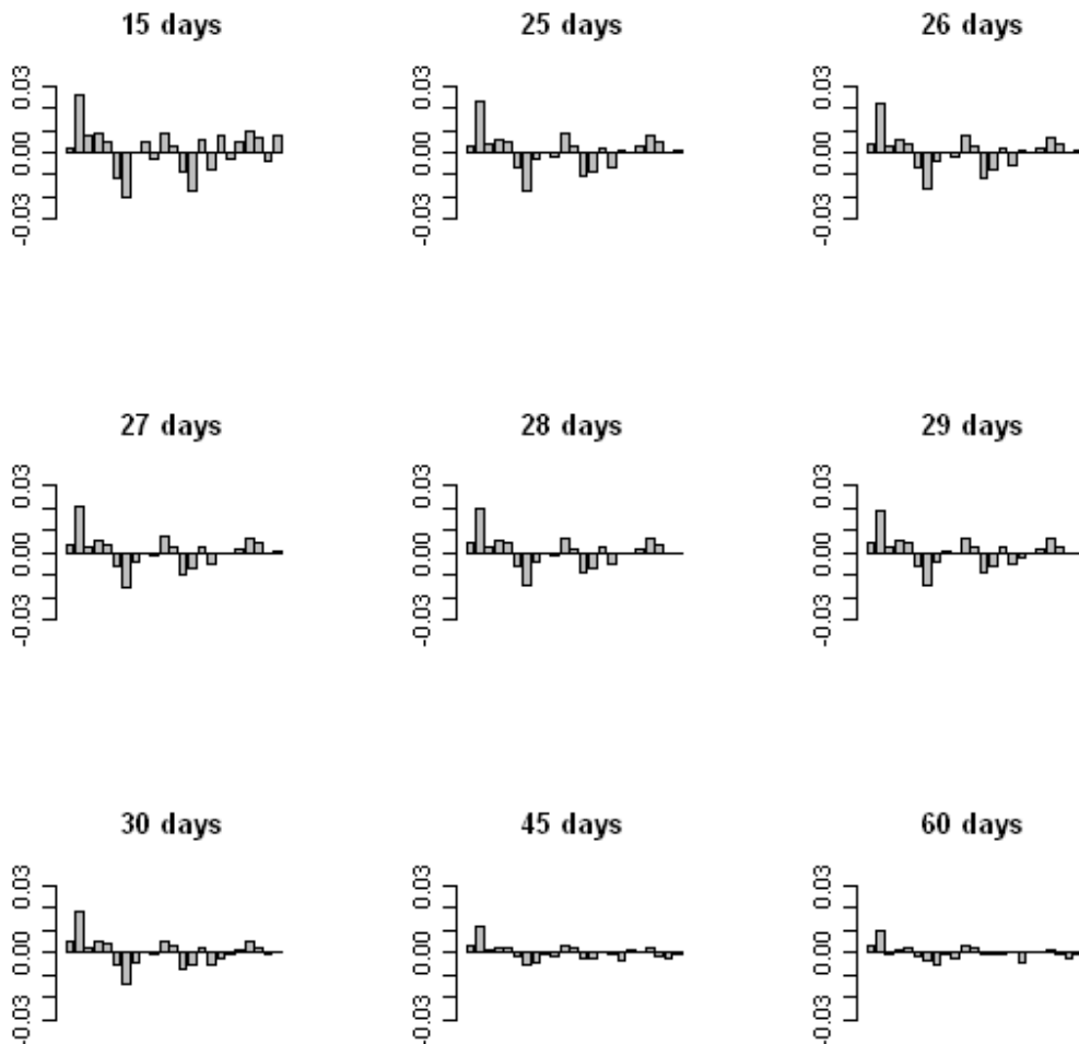
Figure 5.2.1: Unconditional partial indicators at category level for type of business in Industry. Bars represent NACE categories 15 to 37.
