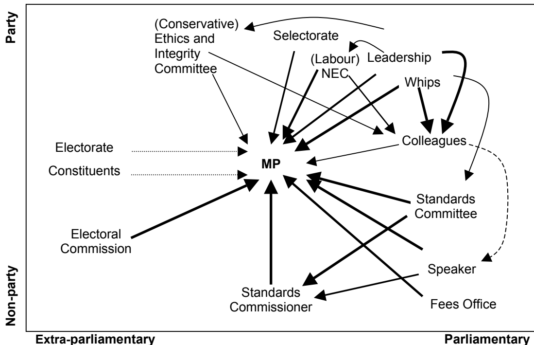
Figure 2: regulatory interrelationships
