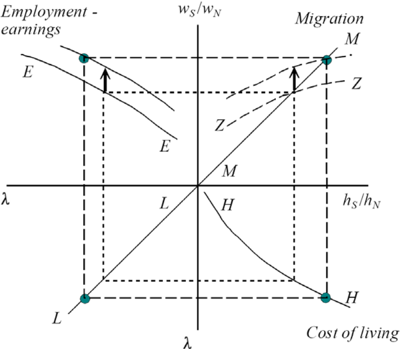
(b) Competing regions
