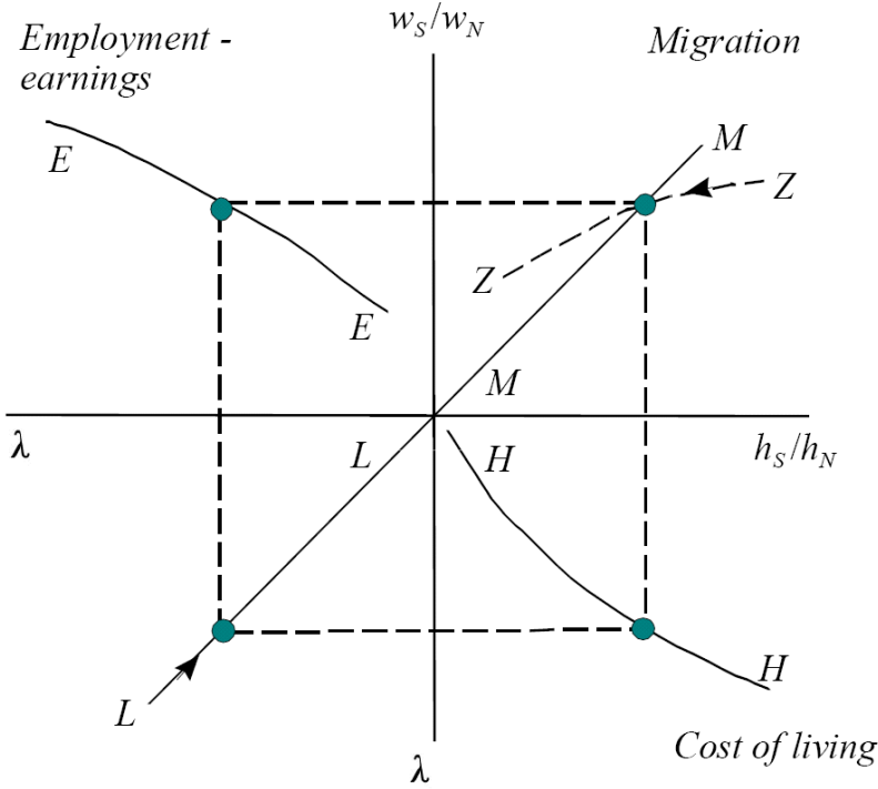
Figure 1: Complementary regions \eta_h > 0 ; \eta_w < 0
