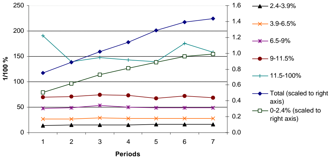
Figure A8. Term structure of the s_{E_j^k} / \hat{L}_j^k ratio for all tranches of the collateral portfolio on the basis of uniform default characteristics of tranches (EVT) for a decreasing forward rate of default (cumulative and periodic loss).
