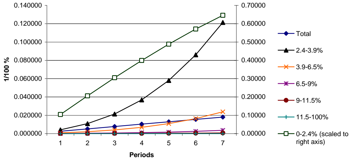
Estimated Loss (logarithmic) (NID/cumulative/constant forward rate)
