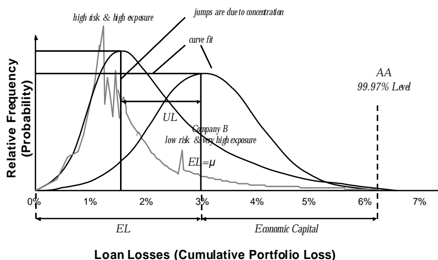
Figure 1. Cumulative distribution function of credit portfolio losses.
