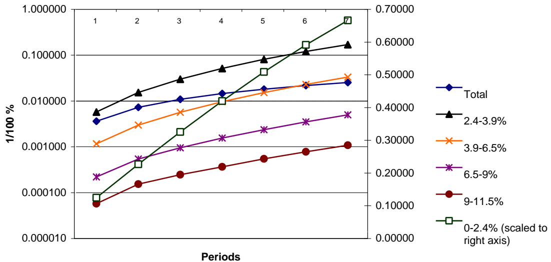
Figure A3. Term structure of cumulative expected losses in various tranches of a collateral portfolio (normal inverse distribution), depicted on a linear and a logarithmic scale. In the linear version of the loss cascades the first tranche [0-2.4%] scales with the right axis. The most senior tranche has been excluded for the logarithmic case due to negative values.
