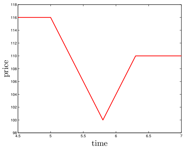
Figure 3: Price dynamics
