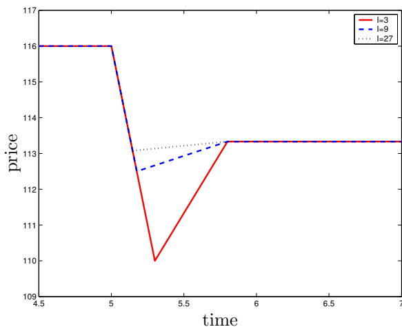
Figure 6: Price dynamics
