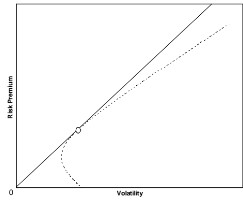
Figure 2: Mean-variance frontiers with and without a safe asset.
