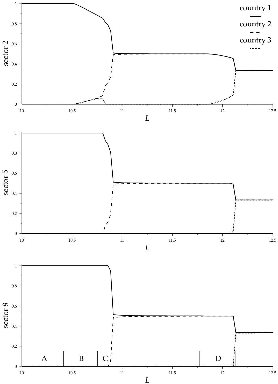
FIGURE 9 Upstream-downstream: share of industry in each country (upstream to downstream from top to bottom panels)
