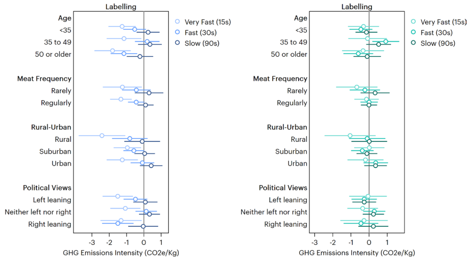
Fig. A4 Additional Heterogeneity Analysis
