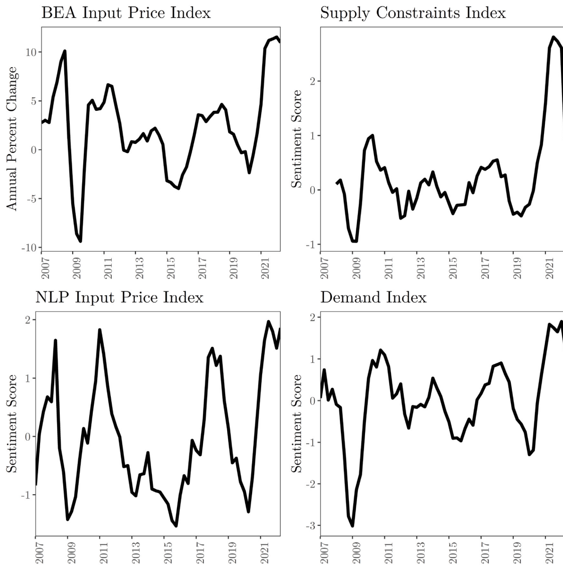
Fig. 4. Independent variables
