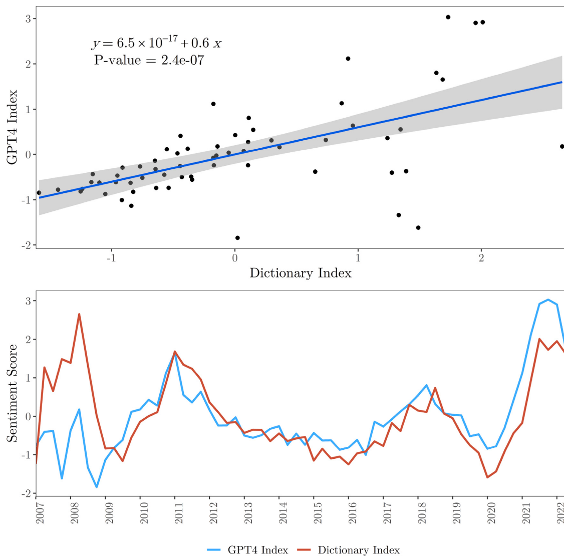
Fig. 2. Cost Increase Sentiment Index: dictionary-based and GPT-based indexes.
