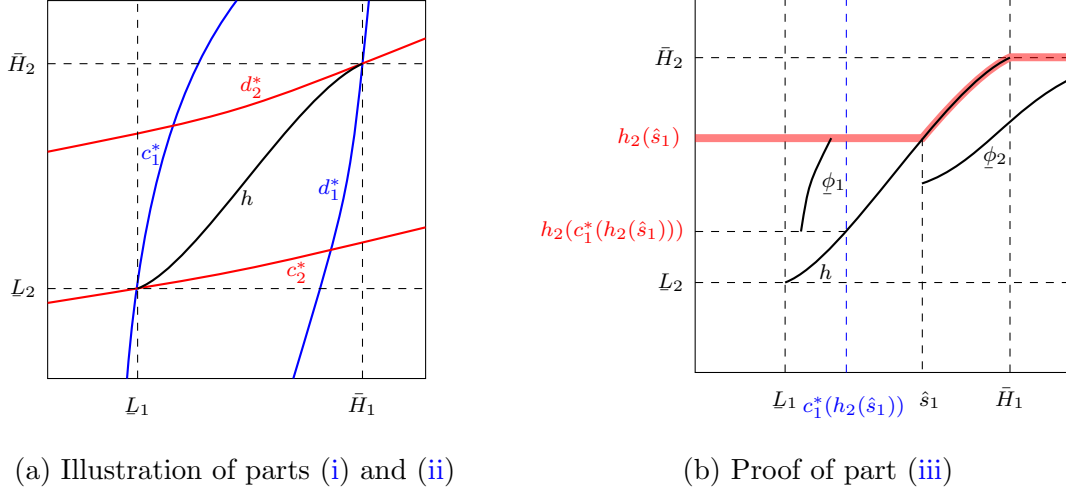
Figure 6: Separation property
