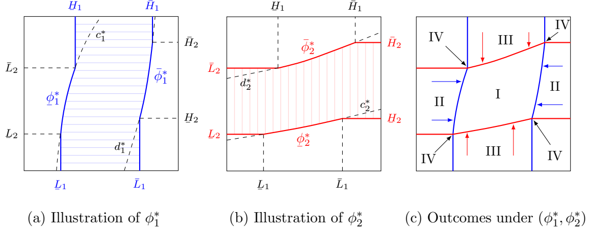
Figure 3: Optimal mechanism
