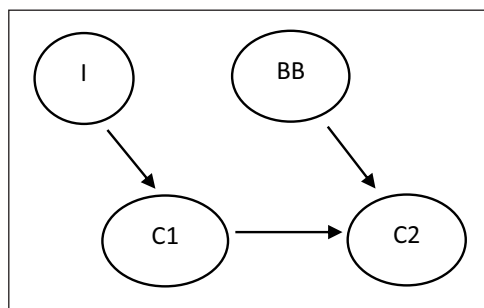
Figure 2: Causal Graph 2
