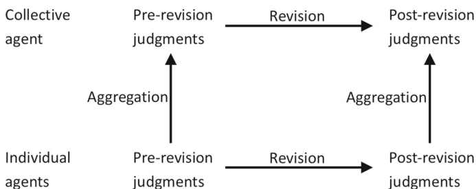
Fig. 1 Aggregation and revision commute
