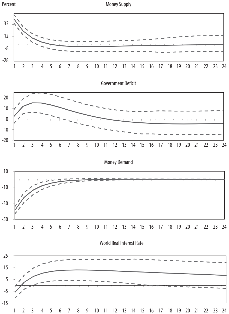
FIGURE 4. Impulse Response of the Index of Market Pressure to Various Shocks during Dual Exchange Regimes a
