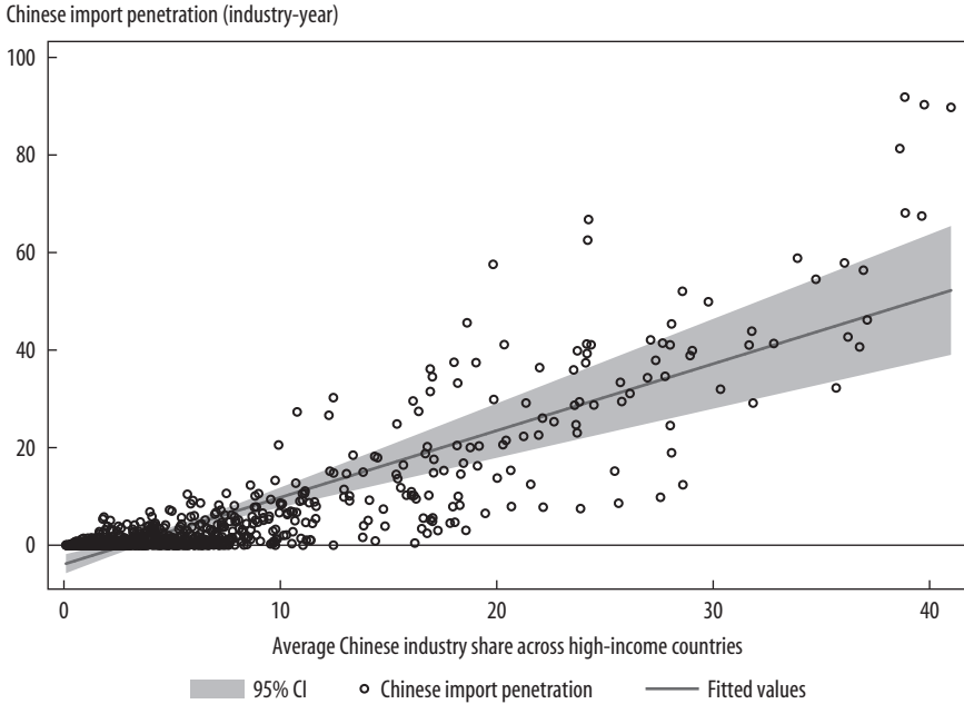
FIGURE 4. First-Stage Correlation
