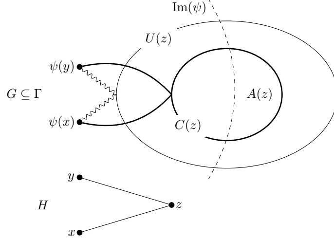
FIGURE 1. Underlying restriction sets, candidate sets, and available candidate sets for an example in which x and y are embedded and their common neighbour z is not. The thick lines are edges of G , and the wavy lines of \Gamma .
