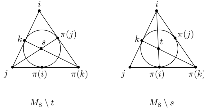
Figure 9: Geometric representations of M_8 \setminus t, M_8 \setminus s (from Case 1 of the proof of Lemma 6.15).
