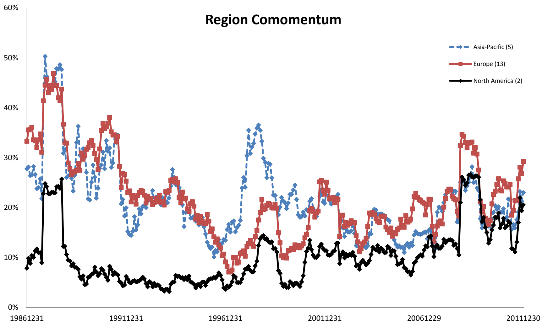
Figure 3: This figure shows the time series of region-specific comomentum measures. At the end of each month, all stocks in a country are sorted into decile portfolios based on their lagged 12-month cumulative returns (skipping the most recent month). Country comomentum is the average pairwise return correlation in the loser decile measured in the ranking month. We calculate region comomentum as the equal-weight country momentum in the region. These regions are Asia-Pacific, Europe, and North America.
