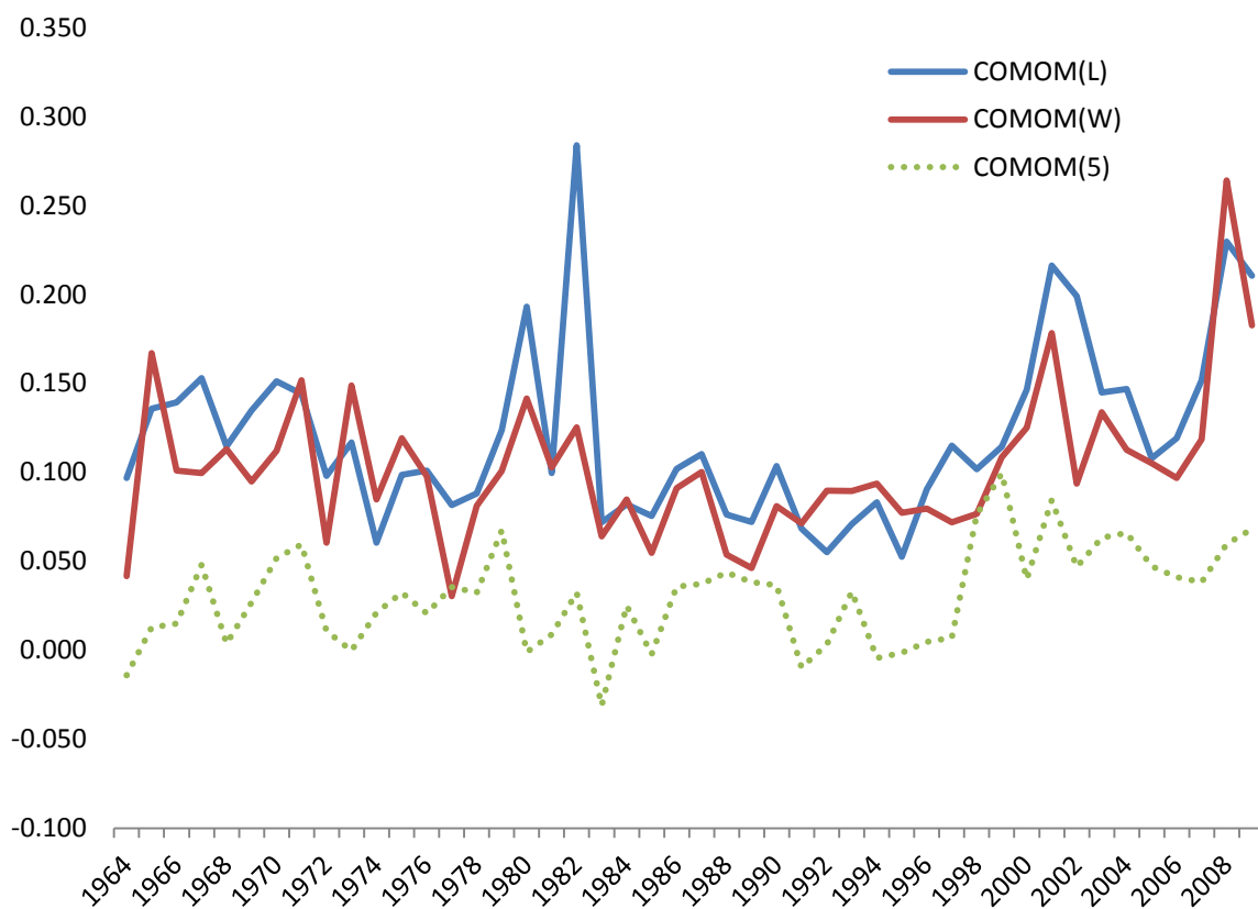
Figure 1: This figure shows the time series of the comomentum measure at the end of each year. At the end of year t-1 , all stocks are sorted into decile portfolios based on their lagged 12-month cumulative returns (skipping the most recent month). comom_L is the average pairwise partial return correlation in the loser decile measured in the ranking year t-1 , comom_W is the average pairwise partial return correlation in the winner decile measured in the ranking year t-1 , and comom_5 is the average pairwise partial return correlation in the median decile measured in the ranking year t-1 .
