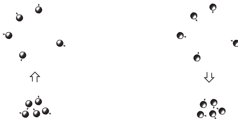
Figure 1.4 Reversing the velocities of a thermodynamic process (left) produces an antithermodynamic process (right).
