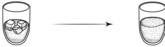
Figure 5.6 The ‘arrow’ of increasing entropy.
