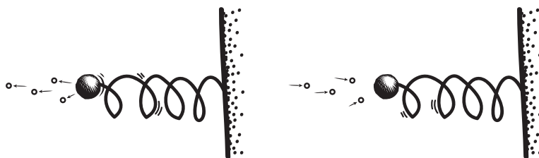
Figure 7.2 A damped oscillator interacts with its microscopic medium (left) in a way that is symmetric under time reversal (right).
