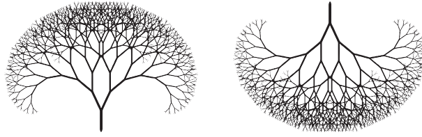
Figure 5.11 Everettian ‘branching’ happens to the future (left) but not to the past (right).
