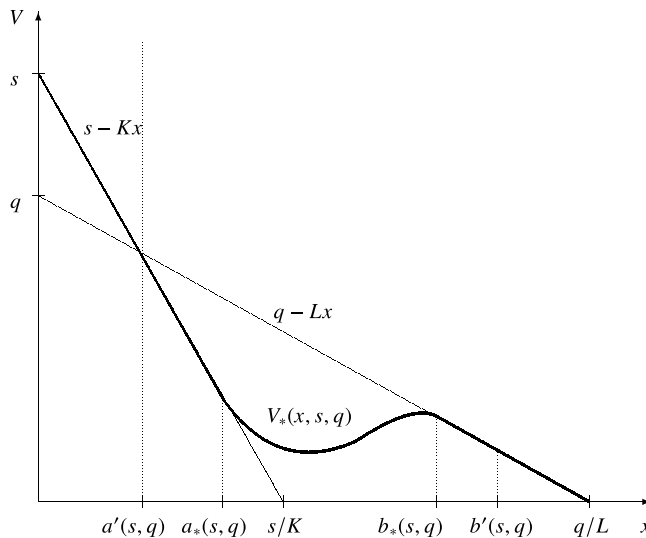
FIGURE 4. A computer drawing of the value function V_*(x, s, q) and optimal exercise boundaries a'(s, q) < a_*(s, q) < b_*(s, q) < b'(s, q) , for each 0 < q < s fixed.
