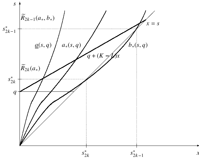
FIGURE 1. A computer drawing of the optimal exercise boundaries a_*(s, q) , b_*(s, q) , and \underline{a}(s, q) , for each q > 0 fixed.
