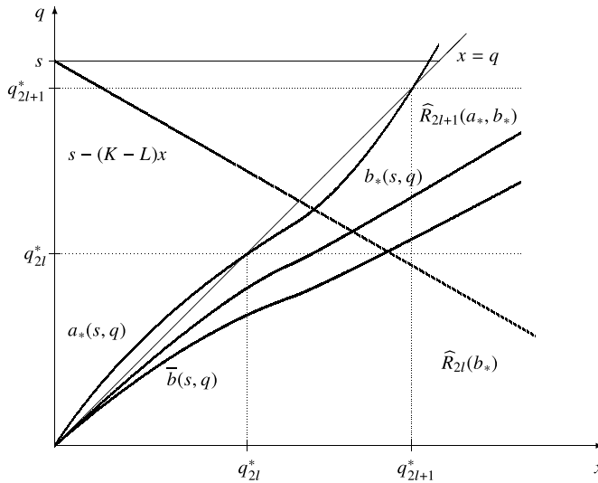
FIGURE 2. A computer drawing of the optimal exercise boundaries a_*(s, q) , b_*(s, q) , and \bar{b}(s, q) , for each s > 0 fixed.
