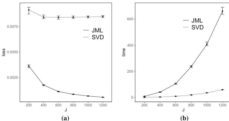
FIGURE 3. Simulation results when K = 4 and the true factors are correlated. The two panels show the same metrics as in Fig. 2
