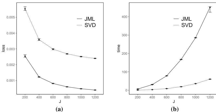
FIGURE 4. Simulation results when K = 8 and the true factors are independent. The two panels show the same metrics as in Fig. 2
