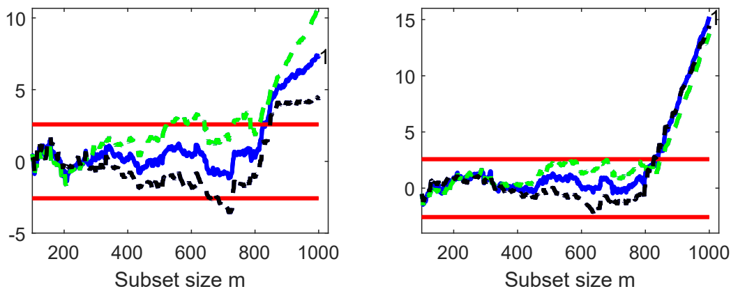
Figure 5: Simulated data. Extended fan plots with green (mostly upper) curve for positive observations: left-hand panel, \lambda_0 = 1 , indicating influential observations and the need for two transformation parameters; right-hand panel, checking \lambda_N = 0.25 and \lambda_P = 1.5 (test of \lambda_0 = 1 for transformed data), confirming transformation parameter values and suggesting the presence of potential outliers.
