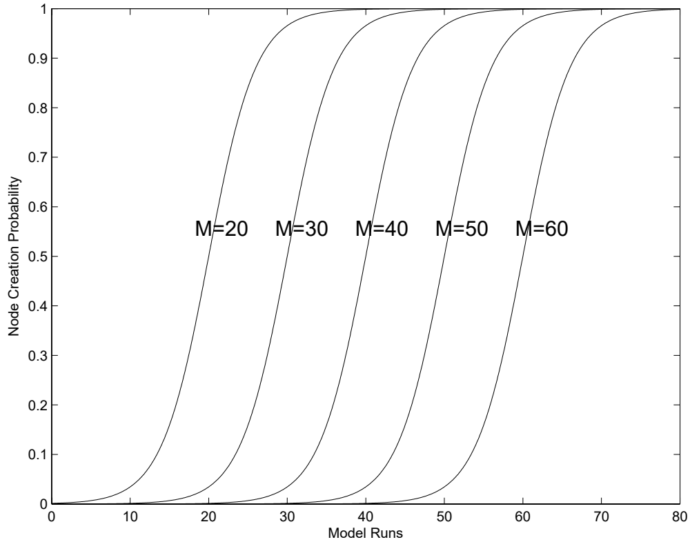
Fig. 3: Differences in the pattern of rate of change in NCP as a function of changes in m has the effect of reducing the rate at which the NCP changes as a function of the amount of input seen, with each increase in t resulting in a decrease in the rate at which the NCP changes (see Fig. 4). Setting the constant t to 3 is therefore simply a convenient way of slowing down learning such that the size of the network, and hence the MLU of the model's output, does not increase so quickly with each exposure to the corpus that it would be necessary to stop the model in mid-run in order to match its MLU to the MLU points of interest in the child data.
