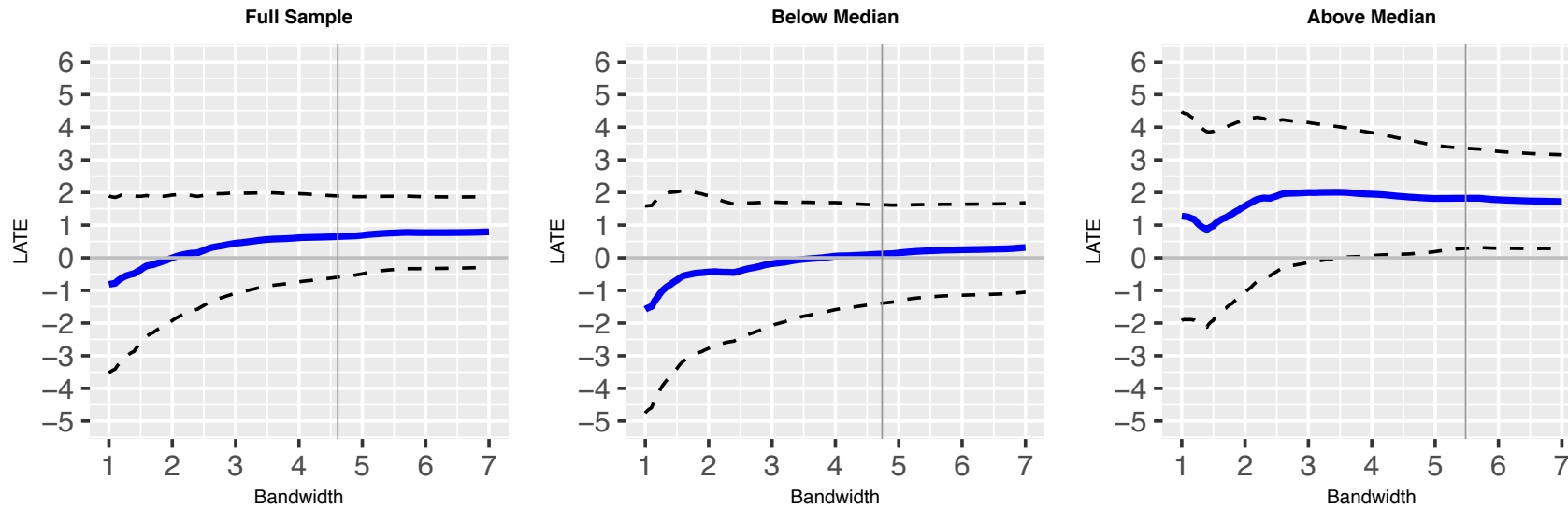
Figure 2: Sensitivity of the Local Linear Regression Estimates to Varying Bandwidth.
