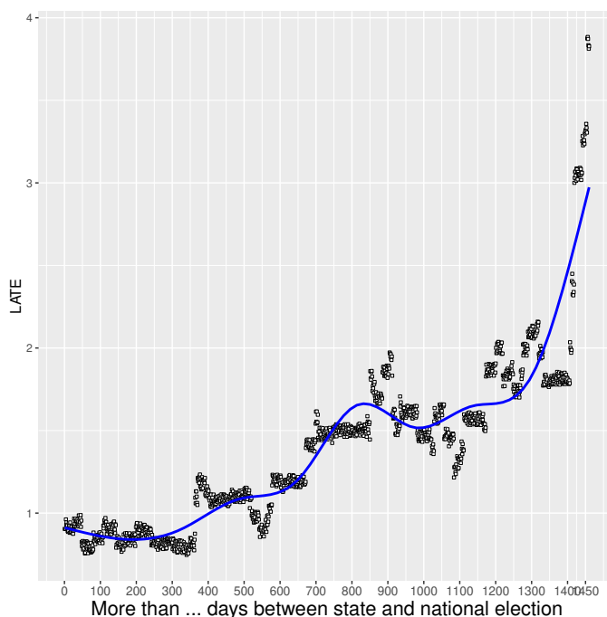
Figure 3: A closer look at the distance between state and federal election and the impact of state representation on federal vote share.
