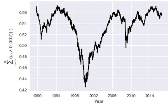
Figure 5. Process \sum_{i=1}^d (\mu_i \wedge 0.002)(\cdot) as a measure of the market diversification degree in the S&P 500 market.
